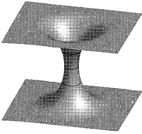
FIGURE 5.2 Foliation of a wormhole by two-spheres.
