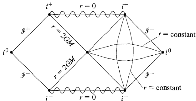
FIGURE 5.16 Conformal diagram for Schwarzschild spacetime.
